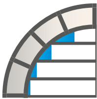
Stepped finish (welded plugs)
